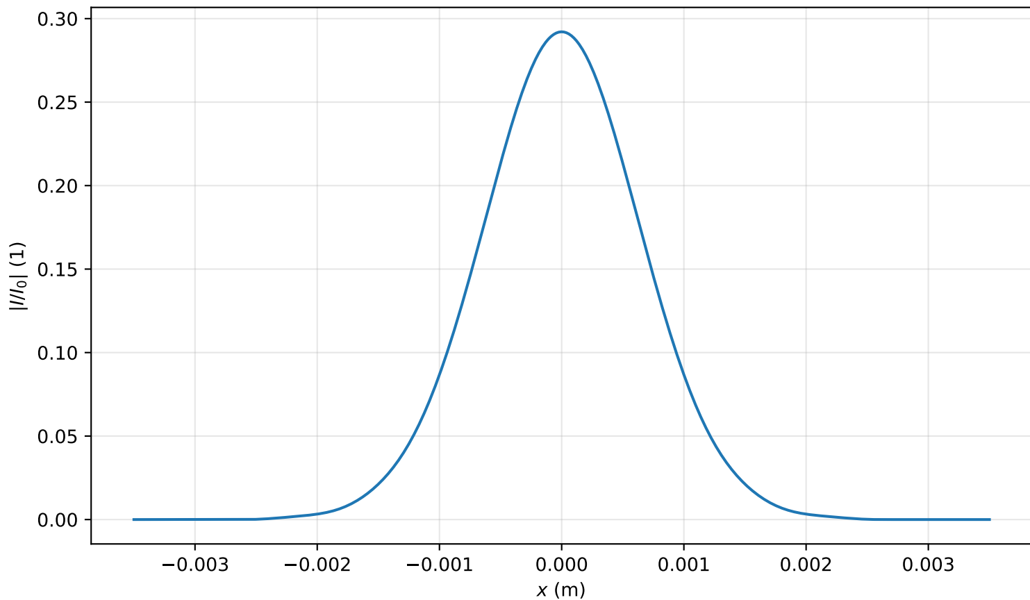
Intensity profile I(x, y = 0, z = 3.582m)/I_0 , P_{in}=0.2P_{cr} , artificial time
